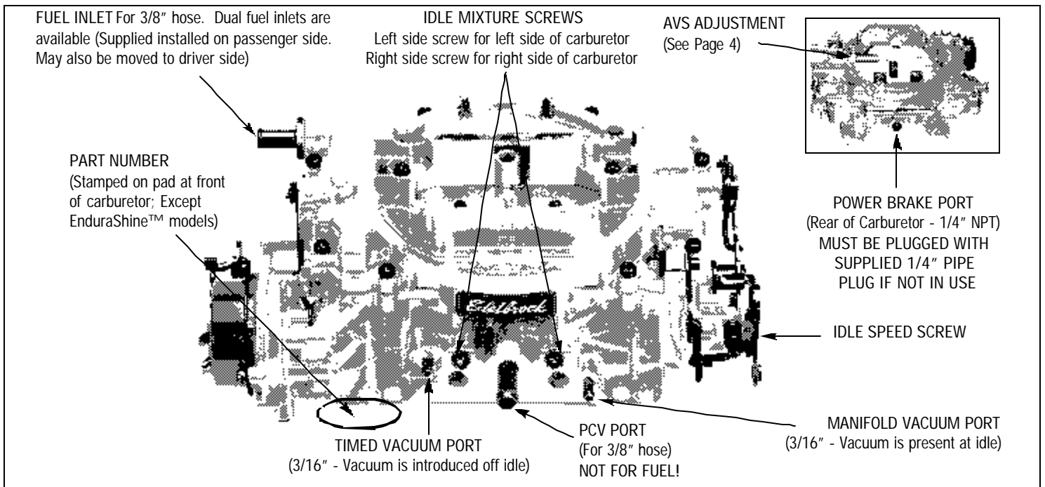
Figure 1 - Fittings and Vacuum Port Location
